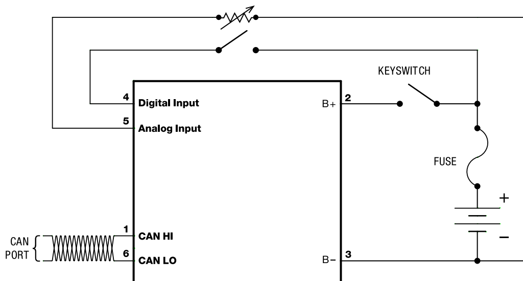
Figure 3. Wiring Diagram
