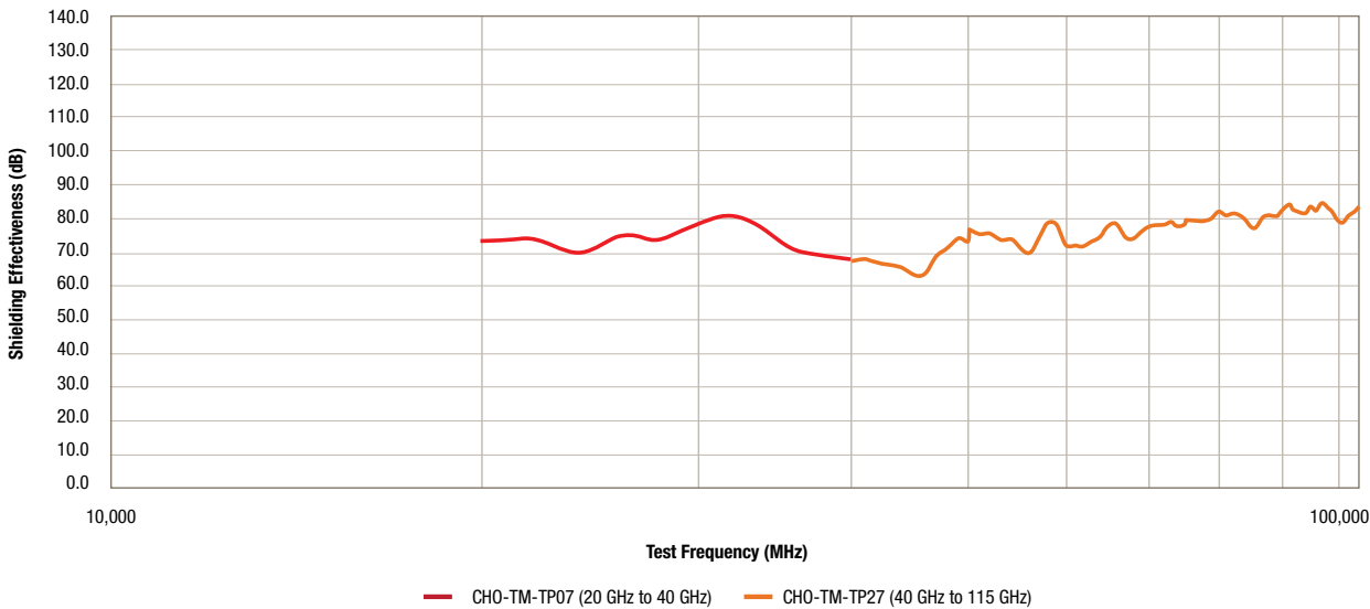
Figure 2 - CHO-SHIELD 2056 Typical Shielding Effectiveness per CHO-TM-TP07 and CHO-TM-TP27
